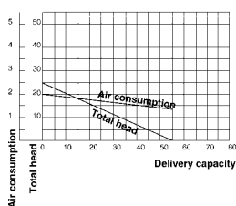
Performance curve YP-18
