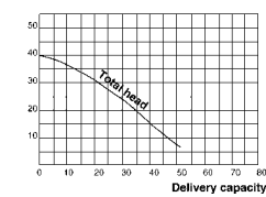
Performance curve YPP-1
