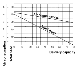
Performance curve YP-35
